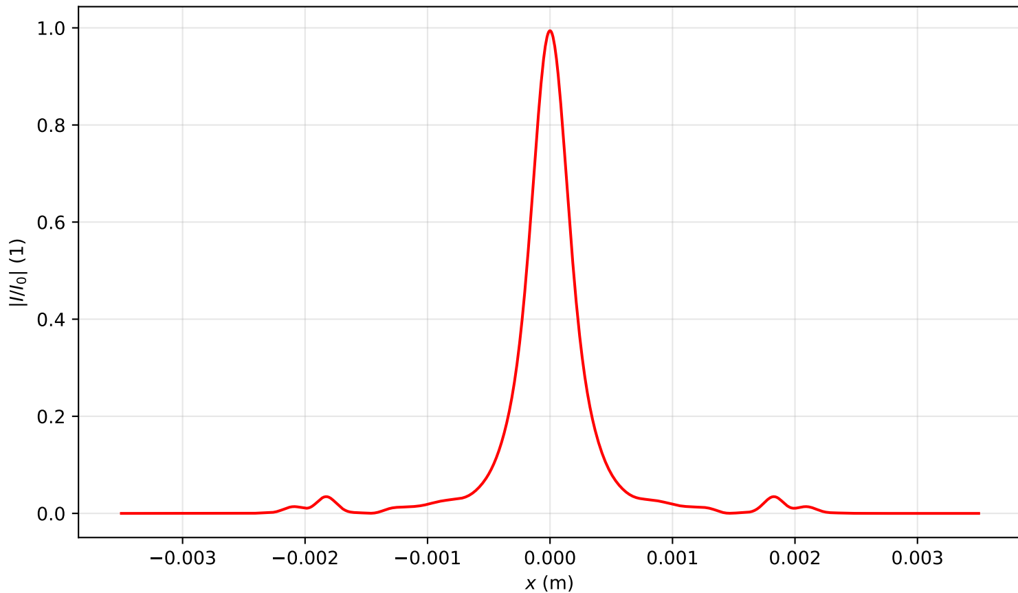
Intensity profile I(x, y = 0, z = 3.582)/I_0 , P_{in}=3.5P_{cr} , artificial time
